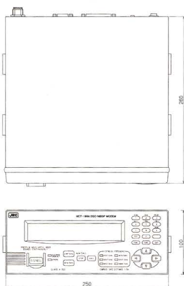
NCT-196N DSC/NBDP Modem
