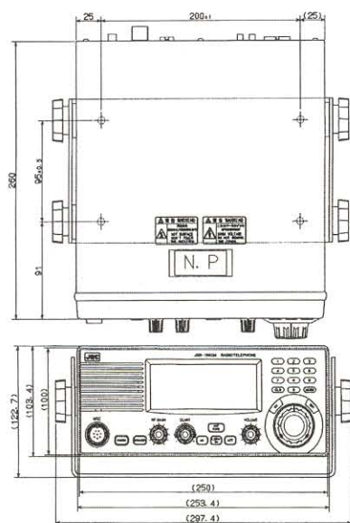
JSB-196GM MF/HF Radiotelephone
