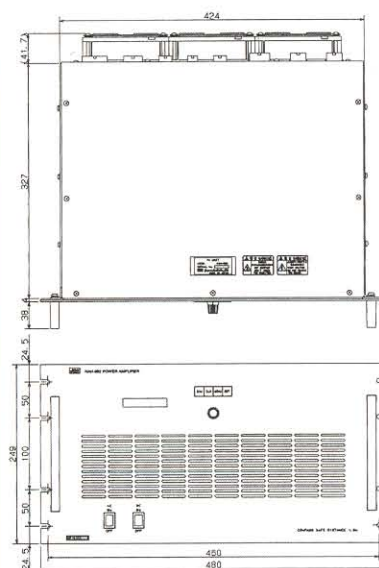
NAH-692/695/698 Power Amplifier
